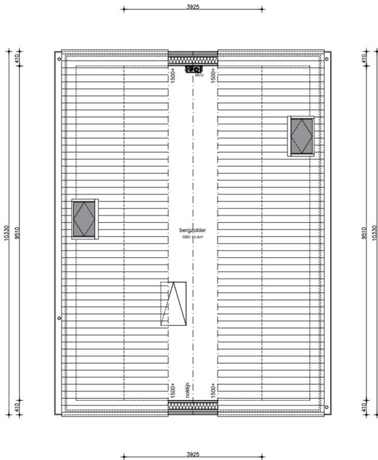
Zolder 1:50
